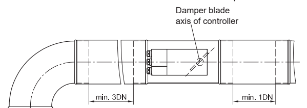
Figure 4: Installation downstream of disruption point, e.g. bend Observe orientation of damper blade axis!
